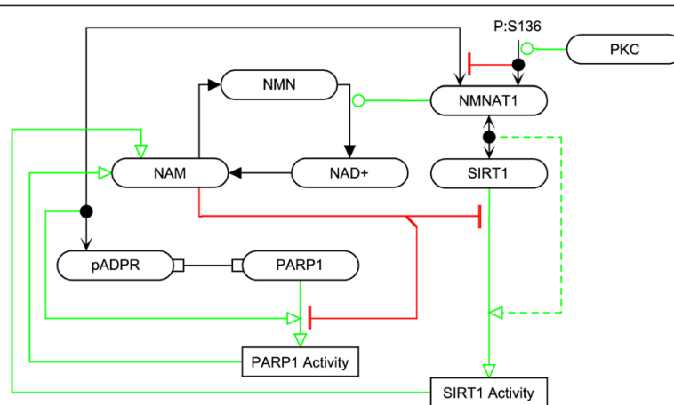
Figure 4 The effect of NMNAT1 binding on SIRT1 and PARP1 activity. Zhang et al. proposed that NMNAT1 may stimulate SIRT1 activity; indicated by the dashed line.
